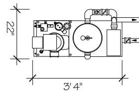
Power Unit & Water Quality System
